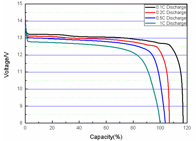
Discharge performance
