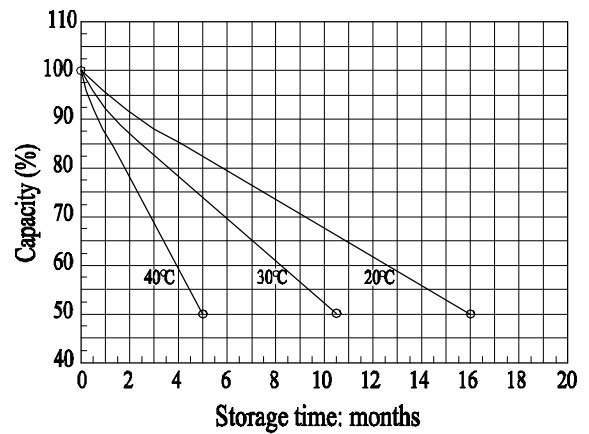
Self-discharge characteristic
